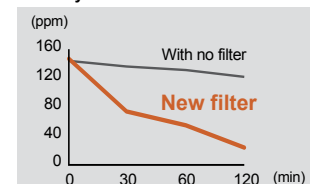
Trimethylamine
