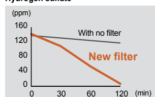
Hydrogen sulfate
